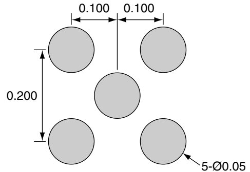
RECOMMENDED FOOTPRINT
